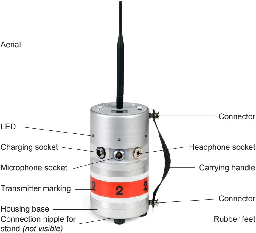
Fig. 1: RT 300 Radio Transmitter
