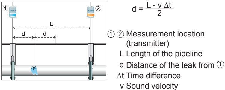
Fig. 3: Principle for determining the leak position
